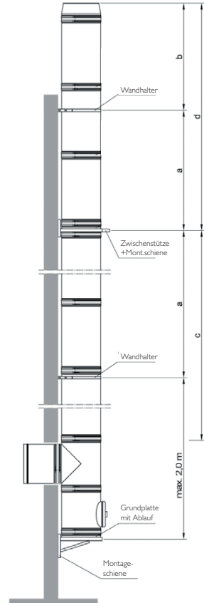
ICS Ø350-700
